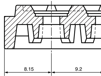
SEC. B-B
