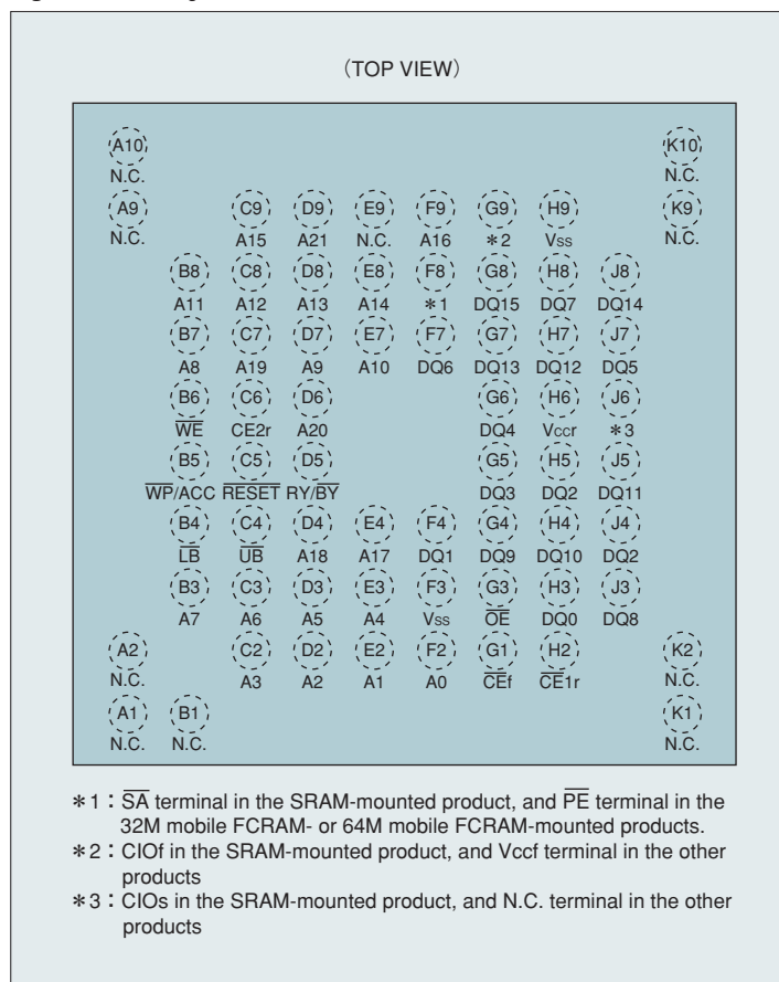
Figure 2 Pin Assignment
